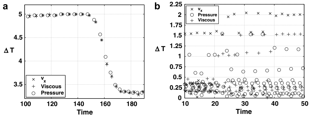
Fig. 7. The characteristic time periods of flapping and rising. Shown are the time intervals \Delta t between consecutive zero crossings in V_x , the pressure force, and the viscous force, for the dynamics shown in Fig. 6. Values are marked at the end point of the interval. These time intervals represent the characteristic periods of the flow–body dynamics. For rising, there is a single characteristic period which undergoes a sharp transition when the amplitude of body oscillations becomes of the order of the chord length. For flapping, there are many characteristic periods, apparently close to integer multiples of the one-half period of flapping. Here a partial transition to longer periods occurs when the horizontal motion becomes of the order of the body chord length.
