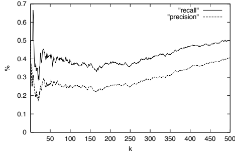
Figure 10: precision-recall measurements
