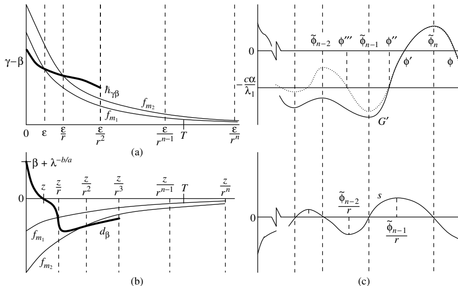
FIGURE 5. Illustrations for the proofs of (a) Lemma 4.8, (b) Lemma 4.10, and (c) Proposition 3.4.
