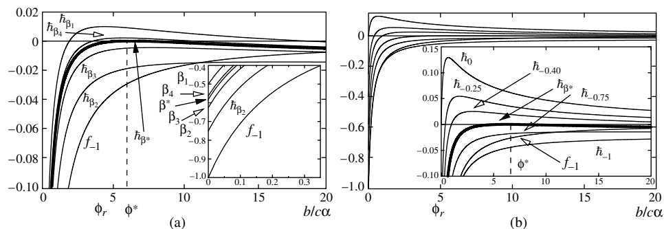
FIGURE 3. Case III. (a) bisection search for \beta^* , (b) comparison of \tilde{h}_\beta(\cdot) for different \beta -values, see (26, 27). For both illustrations, the parameters are \lambda = 1 , \lambda_0 = 3 , \lambda_1 = 1.5 , \alpha = 1 , and c = 0.2 ; we compute r = 1/2 , \phi_d < 0 , \phi_r = 5 , see (13). By Proposition 3.4, \phi_r < \phi^* < b/c\alpha = 20 . The condition (28) on \tilde{h}_{\beta^*} implies that -\lambda^{-b/a} = f_{-1}(0) \leq \tilde{h}_{\beta^*}(0) = \beta^* \leq 0 . Therefore, our search for \beta^* starts in [-\lambda^{-b/a}, 0] = [-1, 0] ; it continues along the intervals [-1, \beta_1] \supset [\beta_2, \beta_1] \supset [\beta_3, \beta_1] \supset [\beta_3, \beta_4] \cdots where \beta_1, \beta_2, \dots are the mid-points of the intervals; the lefthand (righthand, resp.) half of each interval is eliminated if J(\beta) \triangleq \max_{y \in [0, b/c\alpha]} \tilde{h}_{\beta}(y) is negative (positive, resp.). The unique zero of J(\beta) = 0 in [-1, 0] is found after 10 iterations at \beta^* = -0.581 up to three decimal points; J(\beta^*) is attained at y = \phi^* \approx 6.196 . The figure in (b) displays the functions \tilde{h}_\beta for \beta = -1, -0.75, -0.581 (= \beta^*), -0.40, -0.25, 0 . The function \tilde{h}_{\beta^*} is the smallest among all functions \tilde{h}_\beta , \beta \in [-\lambda^{-b/a}, 0] which intersect the y -axis.
