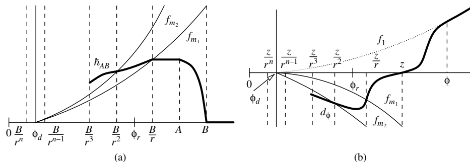
FIGURE 4. Illustrations for the proofs of (a) Lemma 4.1 and (b) Lemma 4.4. The location of \phi_r is unimportant as long as \phi_d < \phi_r < A < B in (a), and \phi_d < \phi_r < \phi in (b).
