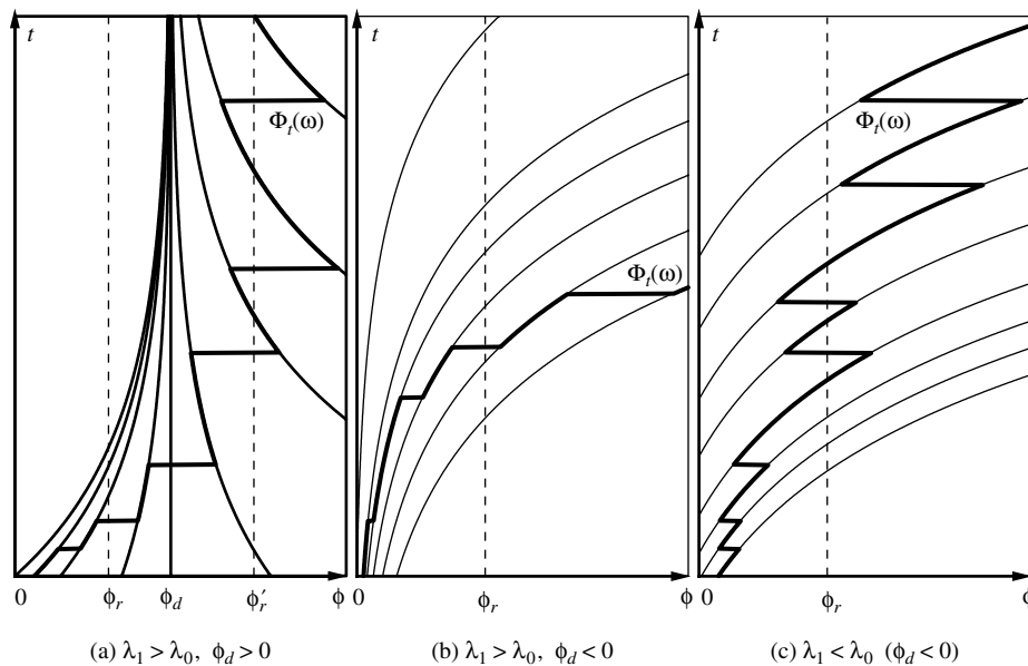
FIGURE 1. Sample paths of the process \Phi of (11, 14). The process \Phi has positive jumps if \lambda_1 > \lambda_0 (a, b), and negative jumps if \lambda_1 < \lambda_0 (c). The paths increase between jumps if \phi_d < 0 (b, c). Note from (13) that \phi_d is always negative if \lambda_1 < \lambda_0 . If \phi_d > 0 , then \Phi reverts to the mean-level \phi_d between (positive) jumps (a).
