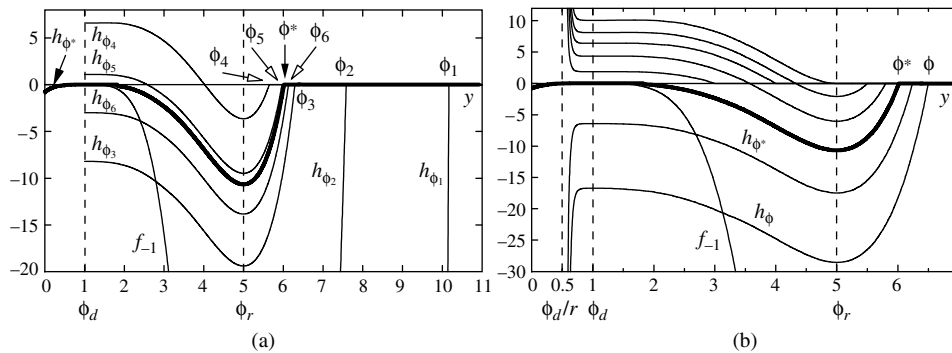
FIGURE 2. Case II. (a) bisection search for \phi^* , (b) comparison of h_\phi(\cdot) for different \phi -values; see (23, 24). For both illustrations, the parameters are \lambda = 1 , \lambda_0 = 3 , \lambda_1 = 6 , \alpha = 1 , and c = 0.2 ; we compute r = 2 , \phi_d = 1 , \phi_r = 5 ; see (13). In (a), the search for \phi^* starts in [\phi_r, \bar{\phi}] = [5, 15.33] with the tight upper bound \bar{\phi} of Proposition 3.3, and continues along the intervals [\phi_r, \phi_1] \supset [\phi_r, \phi_2] \supset [\phi_r, \phi_3] \supset [\phi_4, \phi_3] \supset [\phi_5, \phi_3] \supset [\phi_5, \phi_6] \dots . The mid-points of the intervals are \phi_1, \phi_2, \dots ; the lefthand (righthand, resp.) half of each interval is eliminated if I(\phi_i) \triangleq h_{\phi_i}(\phi_d) is positive (negative, resp.). The unique root of I(\phi^*) = 0 is found at \phi^* = 6.016 up to three decimal points after 17 iterations. The figure in (b) illustrates that the function h_{\phi^*}(\cdot) is the separatrix for (23, 24): among all h_\phi , \phi \in [\phi_d, \infty) , it is the only function bounded between y -axis and y \mapsto f_{-1}(y) of Proposition 3.3. Moreover, h_{\phi^*}(\phi_d) = 0 , and h_\phi(\phi_d) is positive (negative, resp.) for every \phi < \phi^* ( \phi > \phi^* , resp.); the functions g_\phi(y) \triangleq |\lambda + ay|^{b/a} h_\phi(y) explode near y = \phi_d for all \phi but \phi^* . If a + b < 0 , equivalently 1 < r \leq 2 + (2\lambda + \alpha)/\lambda_0 , then only h_{\phi^*} has a stable extension onto \mathbb{R}_+ ; the functions y \mapsto h_\phi(y) above it (below it, resp.) increase to +\infty (decrease to -\infty , resp.) as y decreases to \phi_d/r . (In both (a) and (b), the solutions h_\phi(\cdot) of the differential equation (23, 24) of advanced type are computed by the finite difference method.)
