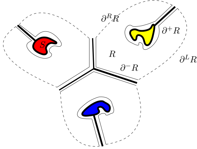
Figure 6: Illustration for Lemma 3.13.
