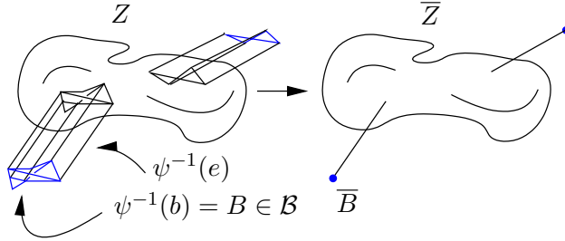
Figure 5: Crushing collars of boundary components.
