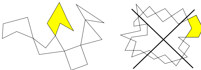
Figure 2: Edge spaces are trees of cylinder cross-sections.
