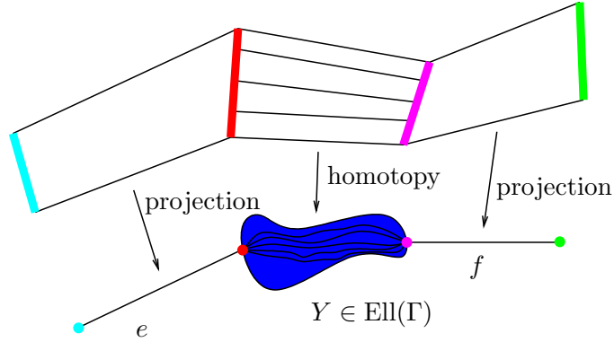
Figure 3: Homotopy between reduced edge paths is a concatenation of rectangles.
