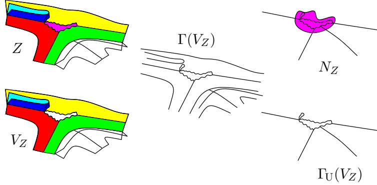
Figure 8: V_Z and all the rest.
