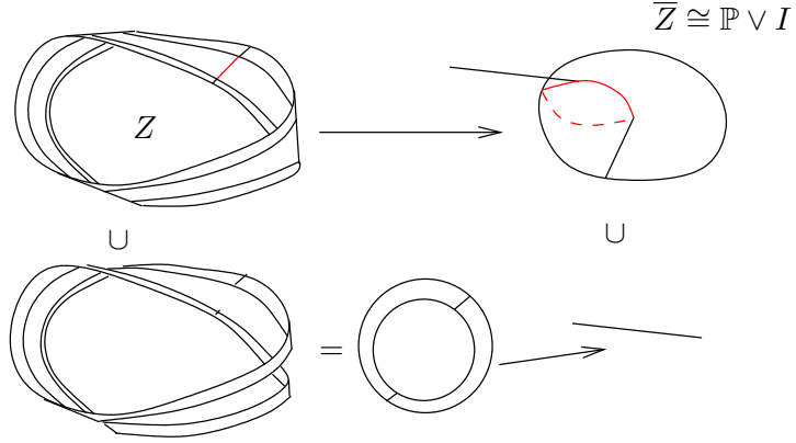
Figure 7: Collapsing a collar neighborhood of a Mobius strip to build a projective plane.
